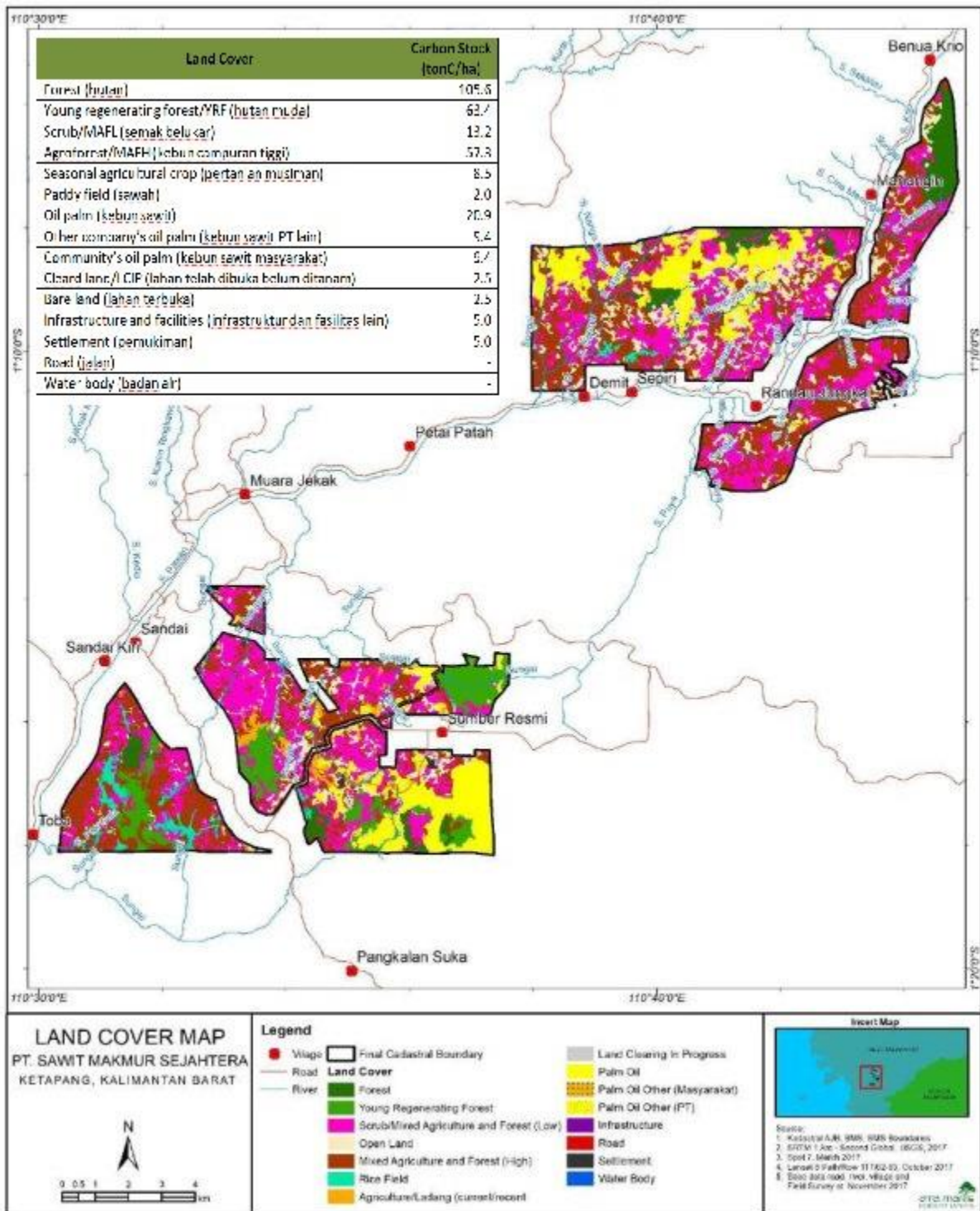
Figure 36. Land cover classification and carbon stock of SMS
