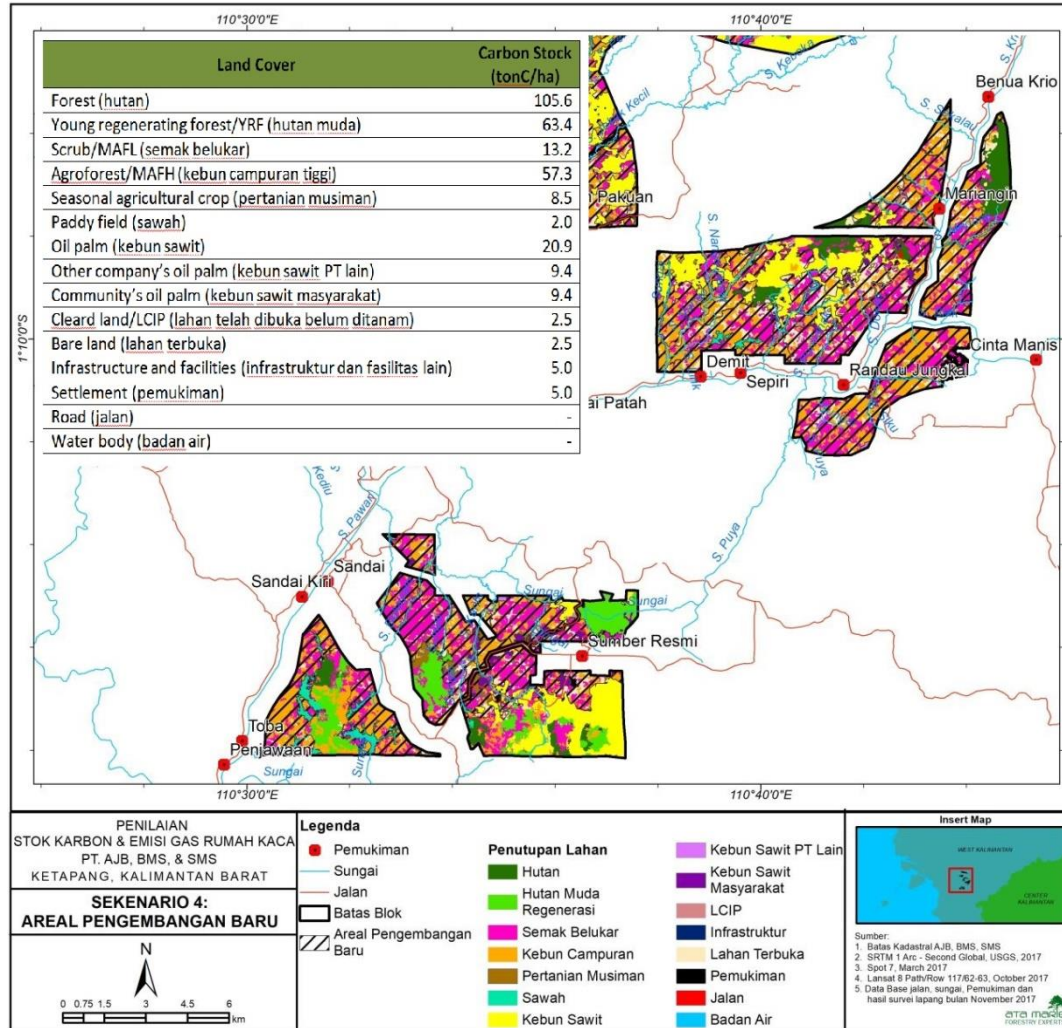
Figure 45. Proposed area for new development in the selected scenario
