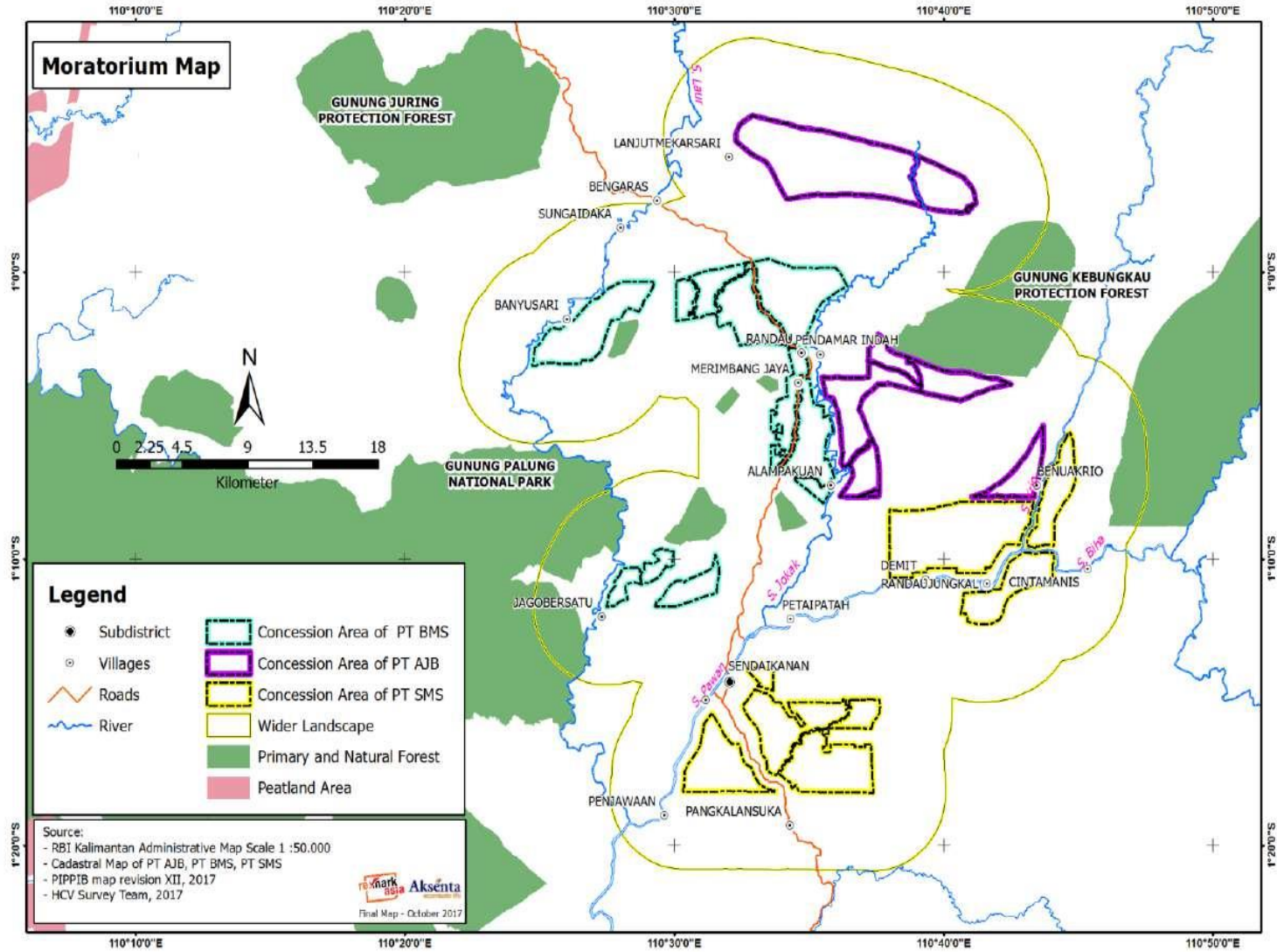
Figure 7. Map showing moratorium areas of primary forest and peatland
