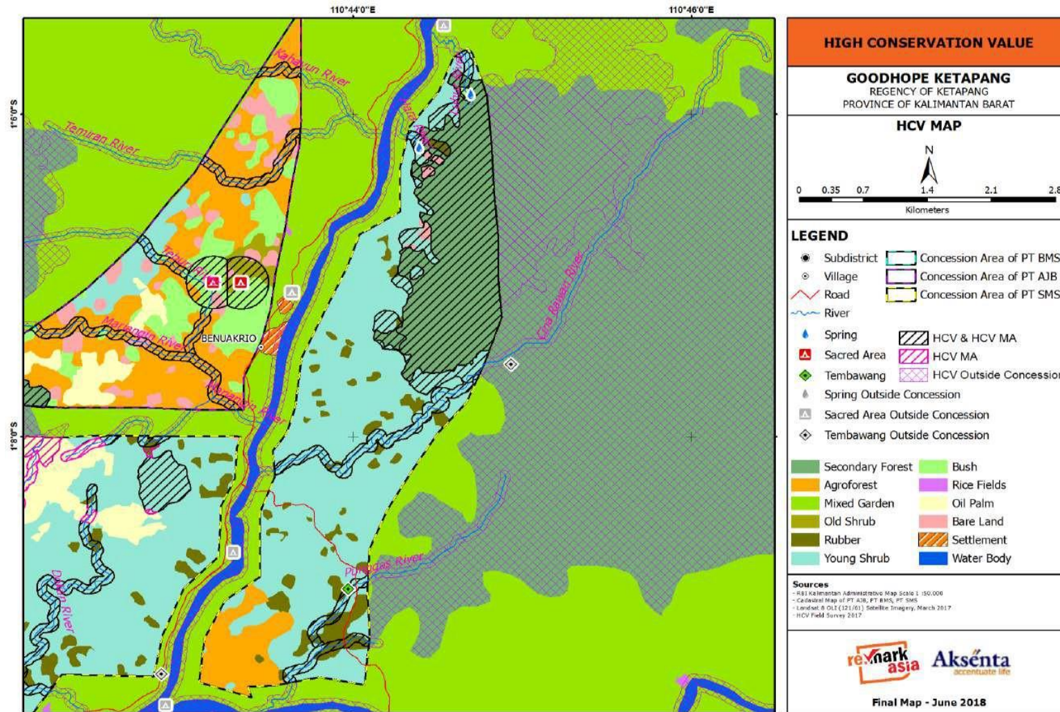
Figure 15. Map of HCVAs and HCVMA in Agro Makmur Estate Area (Eastern Part) - PT SMS
