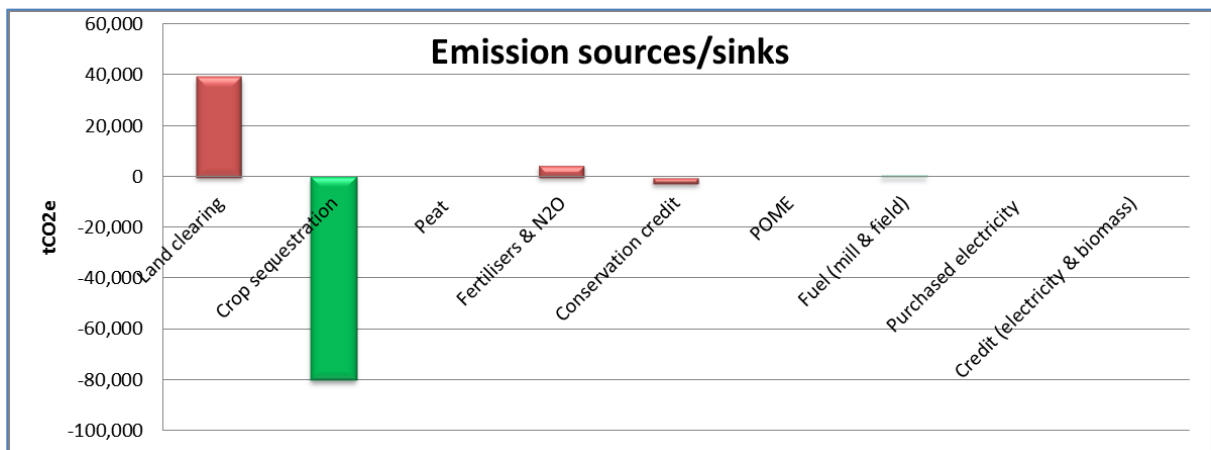
Figure 42. GHG emission amount per source from scenario 2
