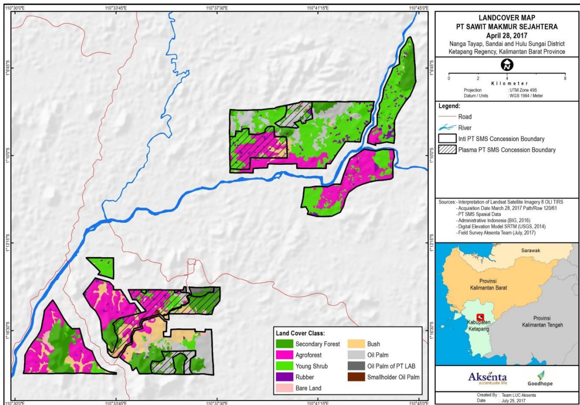
Figure 31. Land cover in April 2017
