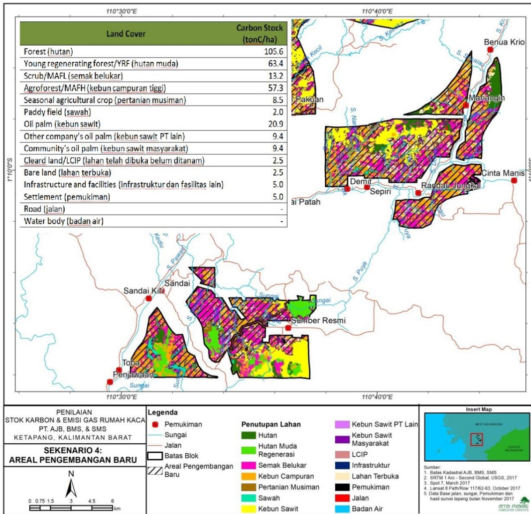
Figure 50. Map showing new development area of SMS
