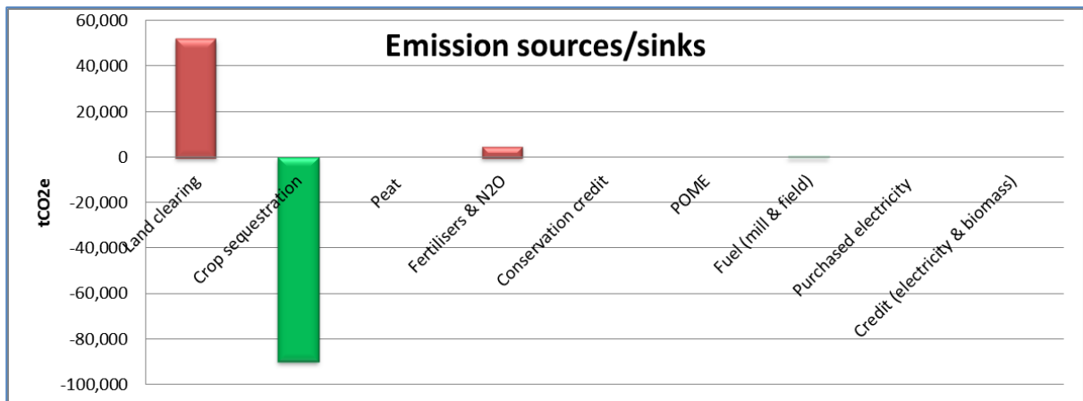
Figure 41. GHG emission amount per source from scenario 1
