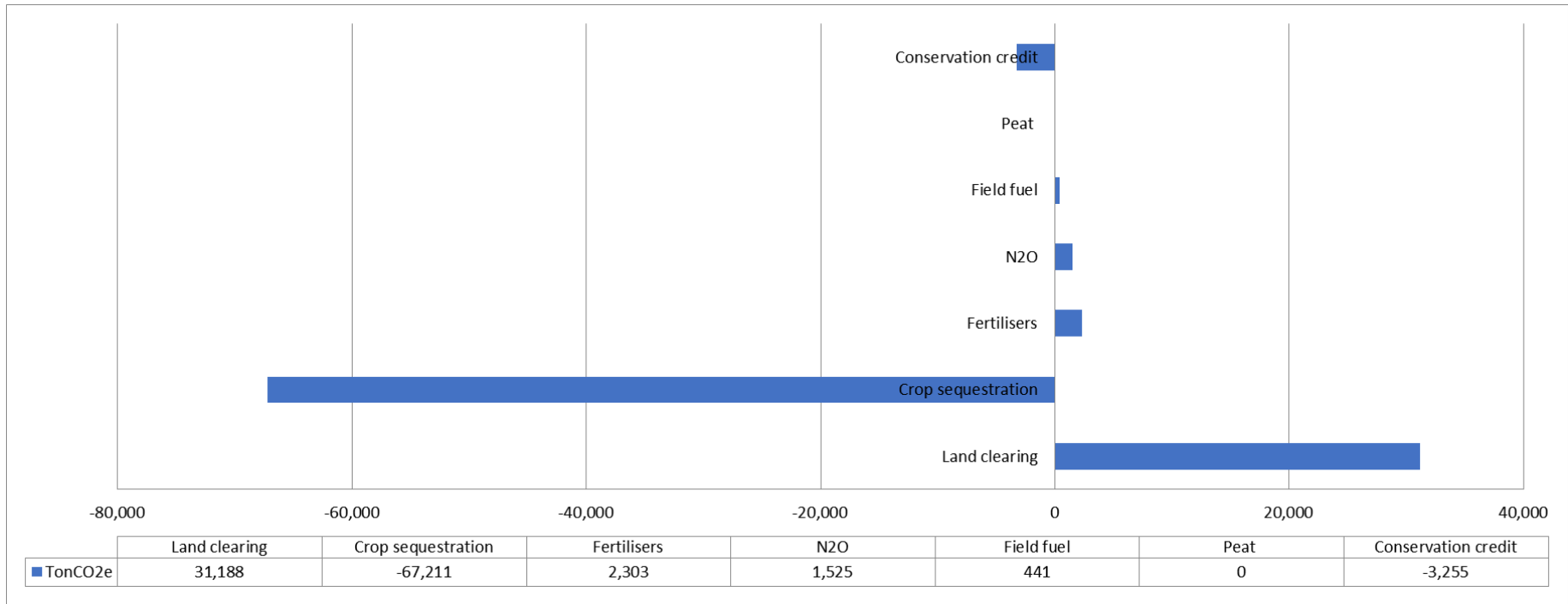
Figure 46. Summary of GHG emission based on sources in the selected scenario
